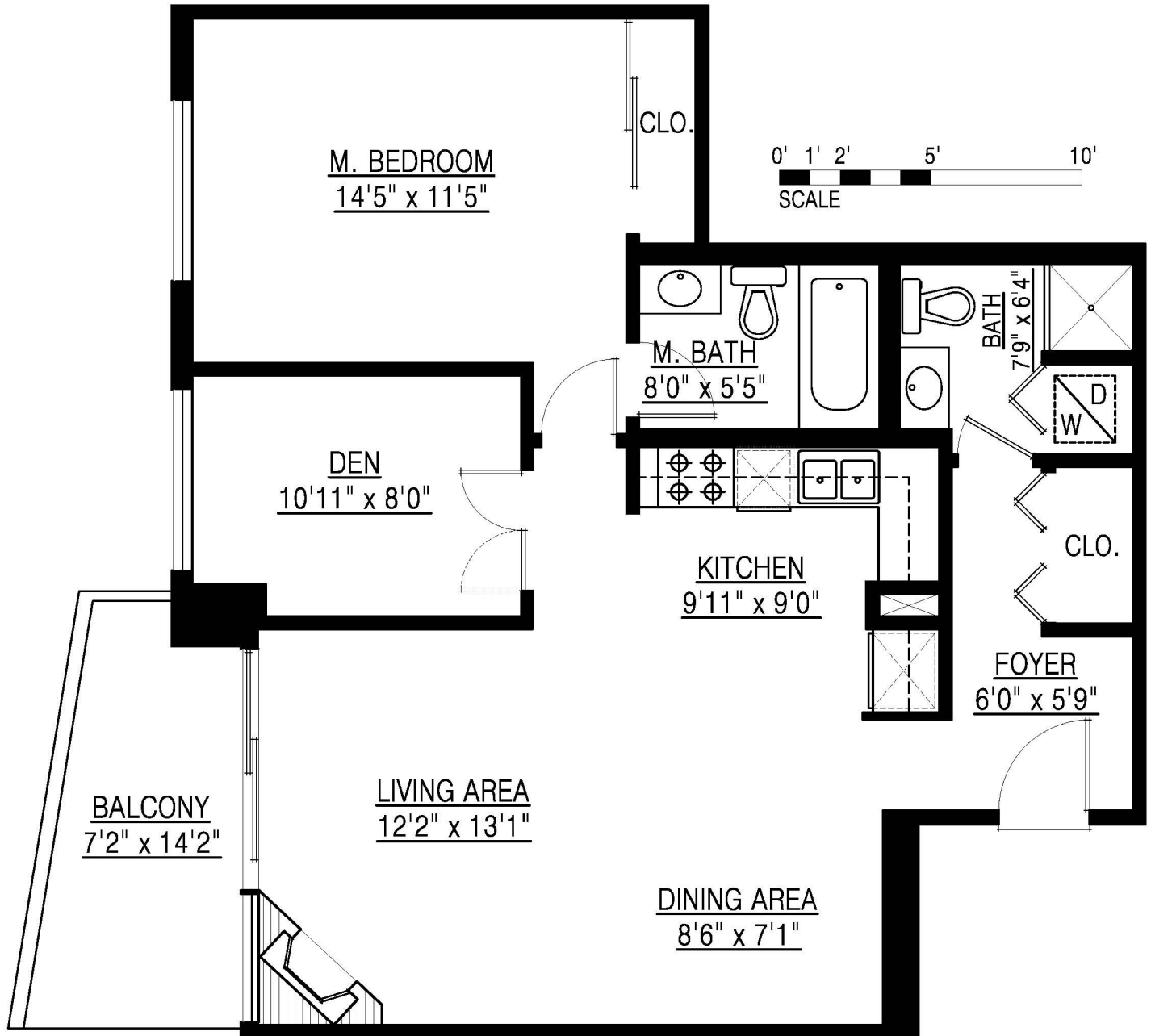
MAIN FLOOR PLAN FLOOR AREA: 880 sq.ft.
