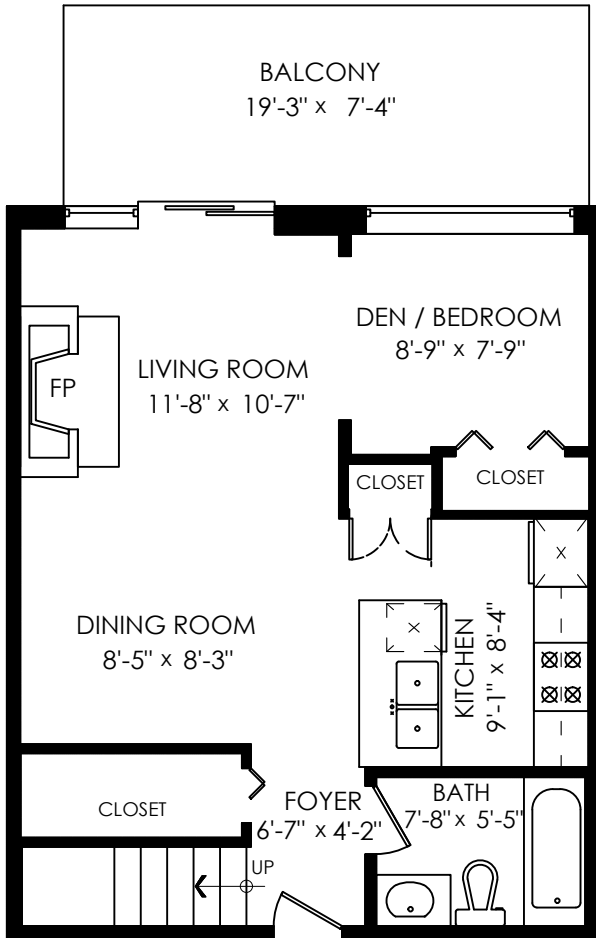
Main Floor: 585 Sq.Ft. Ceiling Height: 7'-10"
